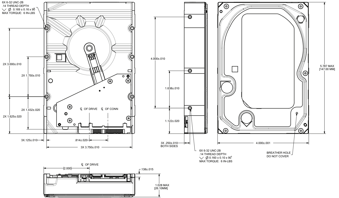
Figure 4. Mounting configuration dimensions 8TB & 6TB models
